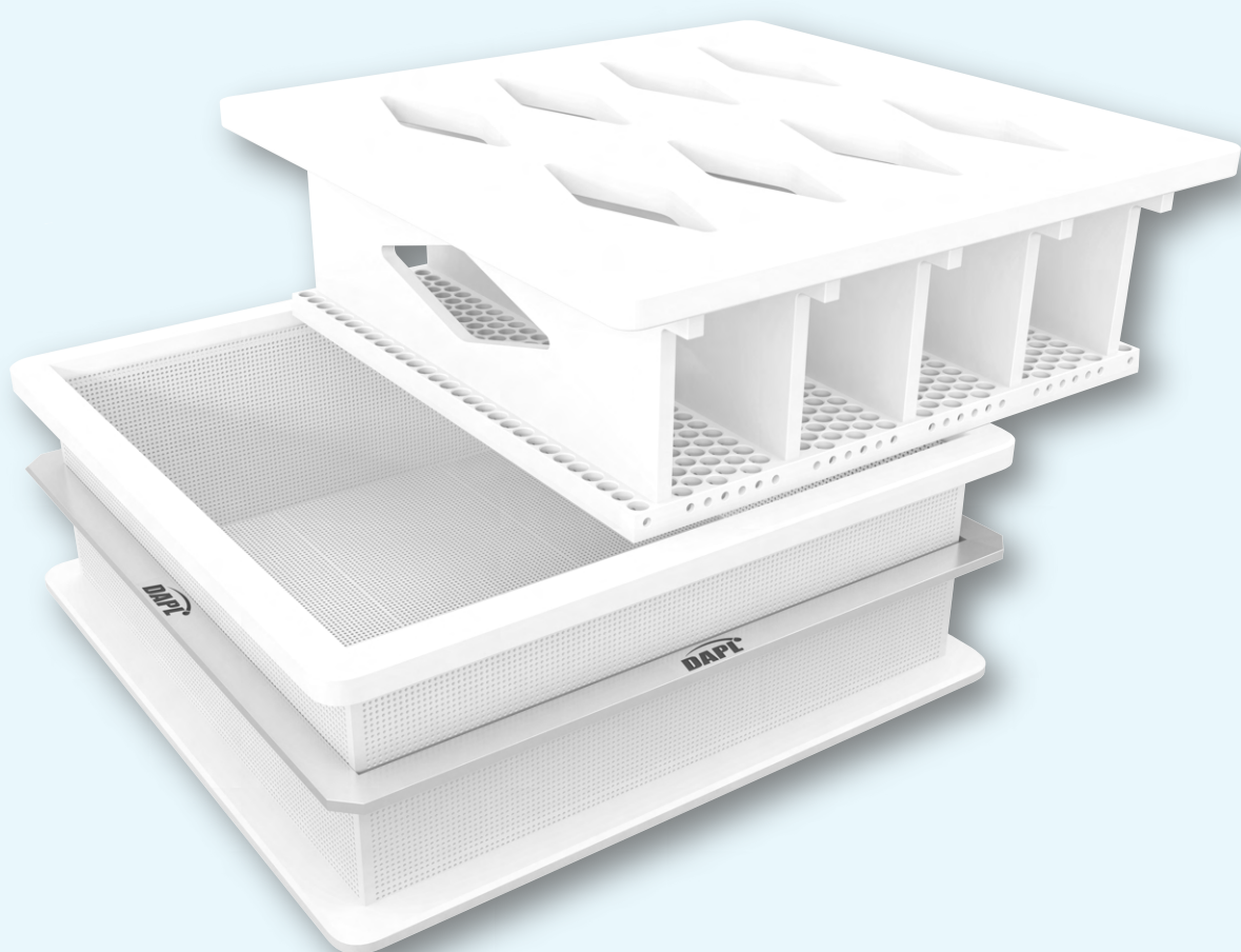
Square Mould
